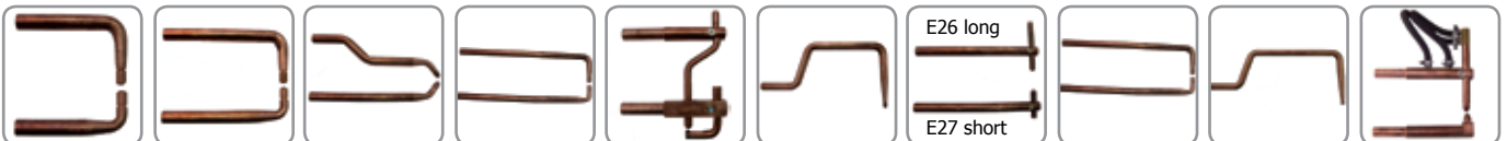
B13 130mm B1 200mm B2 300mm B3 400mm B4 200mm B5 400mm B10 250mm B11 500mm B12 B500 Water Cooled Arms
